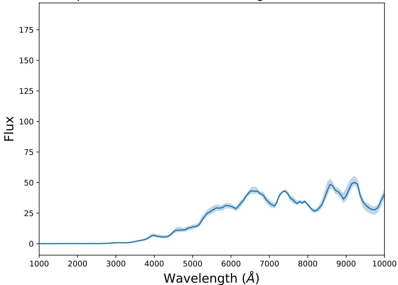
Spectrum 10 for transient 91bg-like at z=0.67
